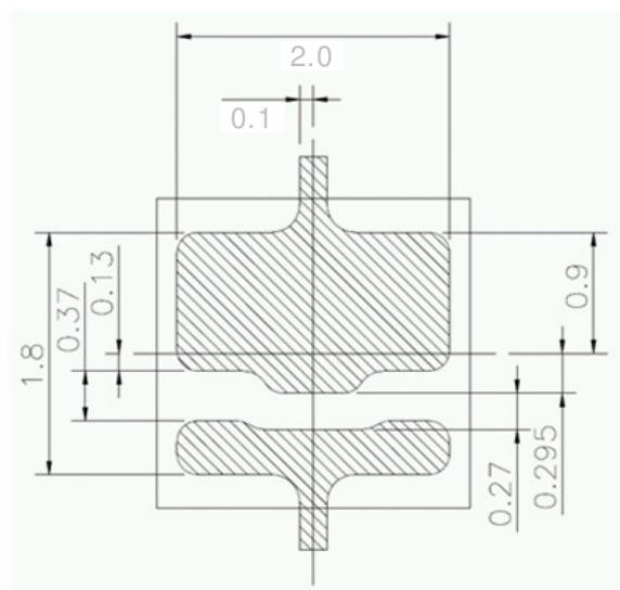
Recommend Land Pattern
